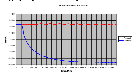
Typical performance freezer unloaded, full cold
