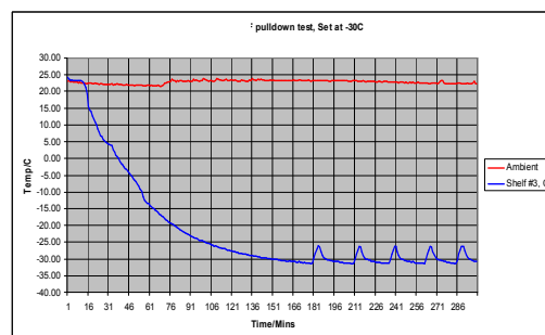
Typical performance freezer unloaded, set point @ -30C
