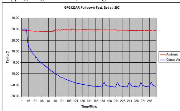
Typical performance air temp pull-down
