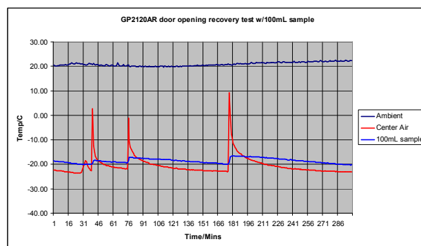
Typical performance, door opening recovery
