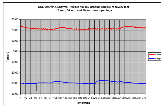
Typical performance, door opening recovery
