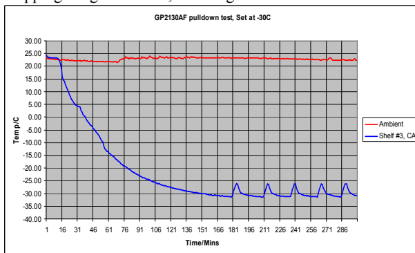
Typical performance air temp pull-down
